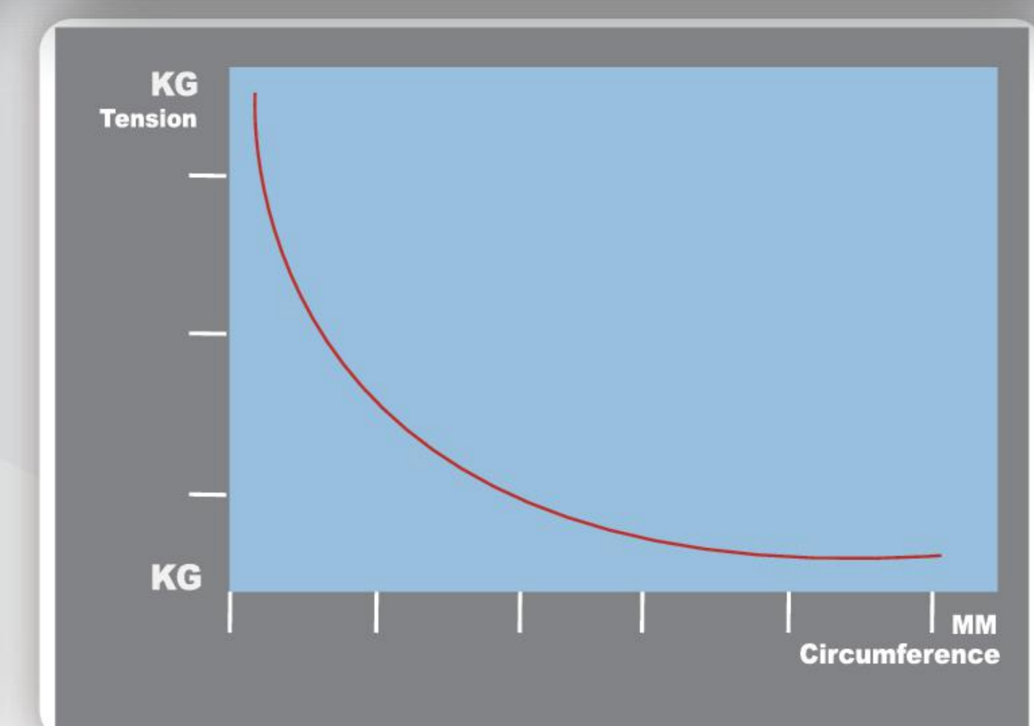
Rewind taper tension function
